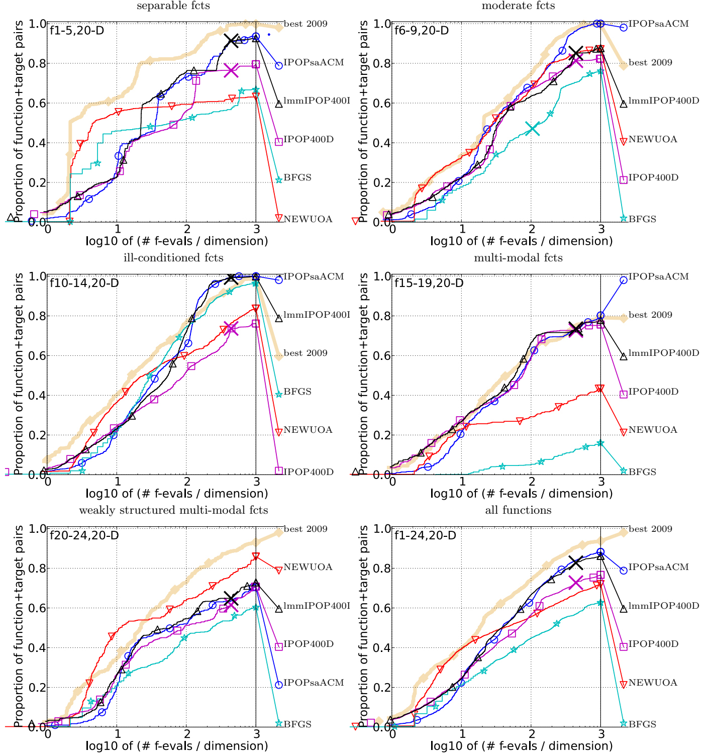
Figure 3: Bootstrapped empirical cumulative distribution of the number of objective function evaluations divided by dimension (FEvals/D) for 31 target f -values just not reached by the artificial GECCO-BBOB-2009 best algorithm within 31 reference budgets in [0.5 \dots 50] \times \text{DIM} for all functions and subgroups in 20-D. The “best 2009” line corresponds to the artificial GECCO-BBOB-2009 best algorithm, i.e., the best ERT observed during BBOB 2009 for each single target.
