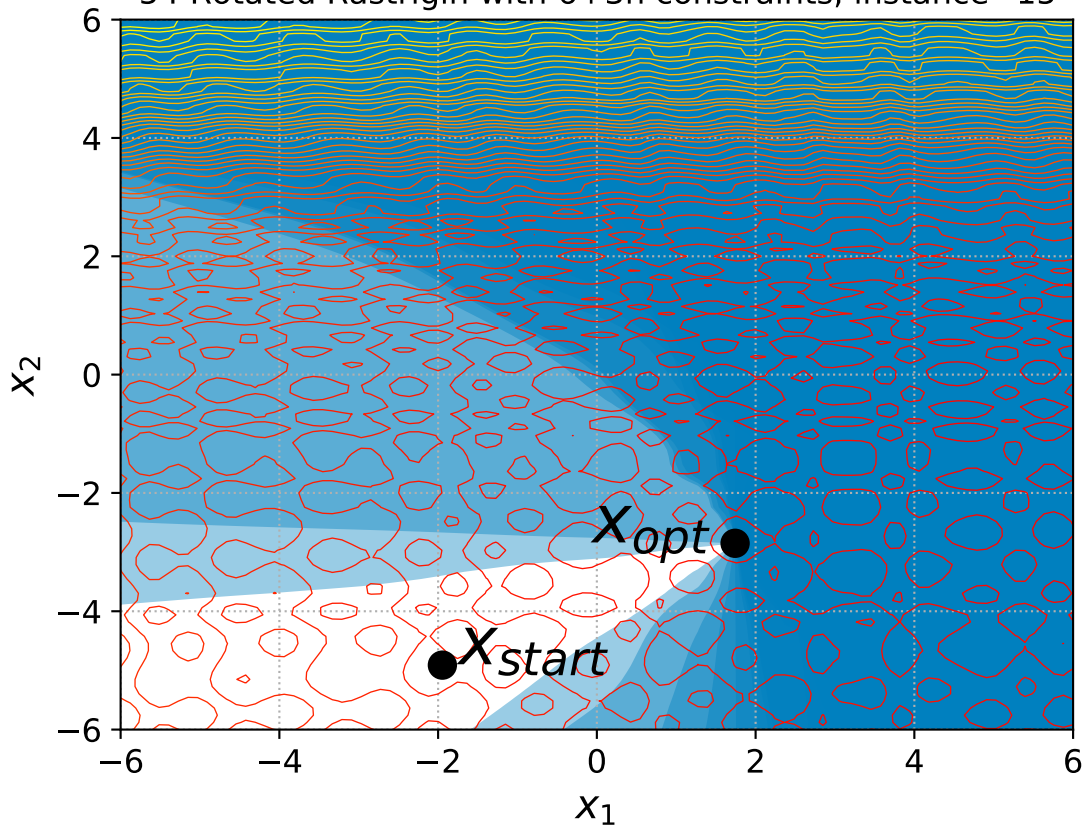
54 Rotated Rastrigin with 6+3n constraints, instance=15
