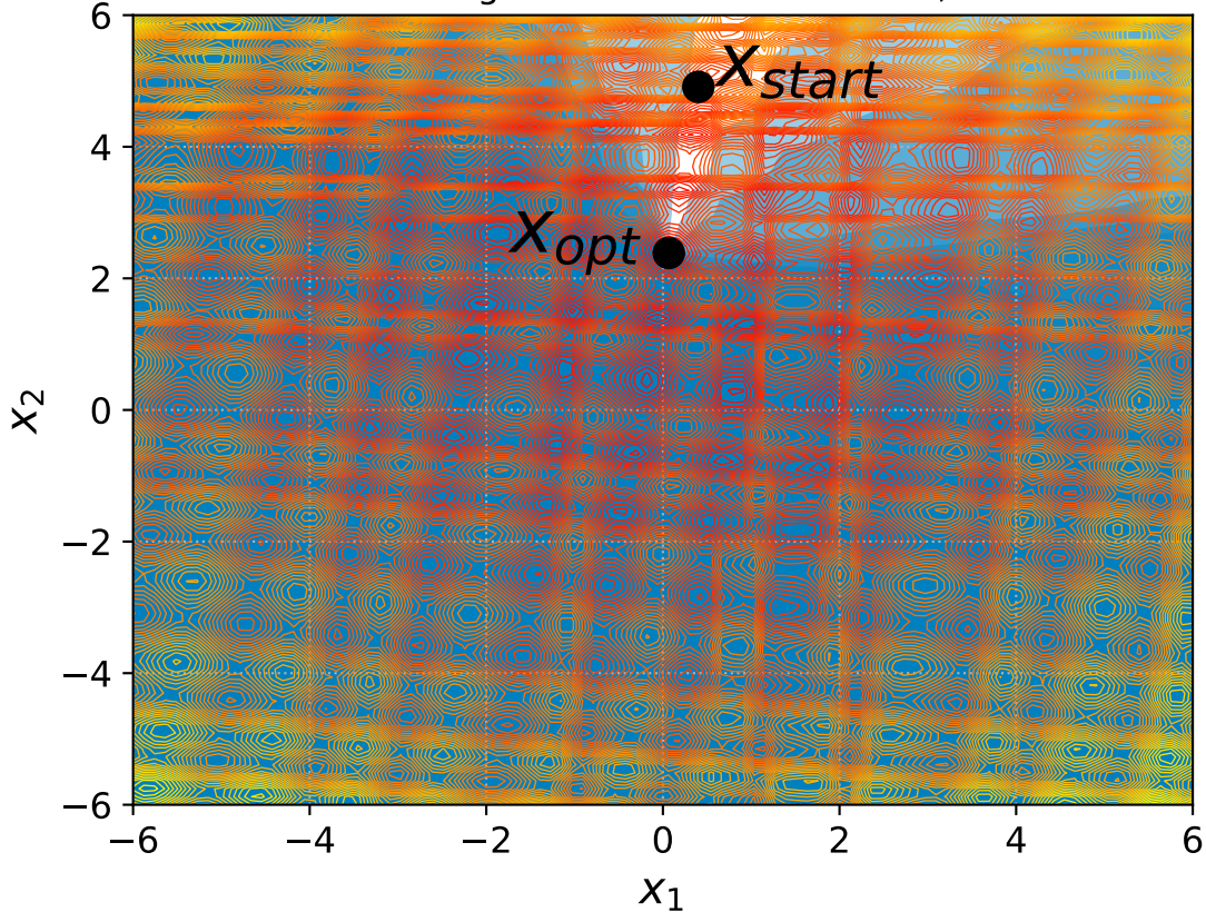
54 Rotated Rastrigin with 6+3n constraints, instance=7
