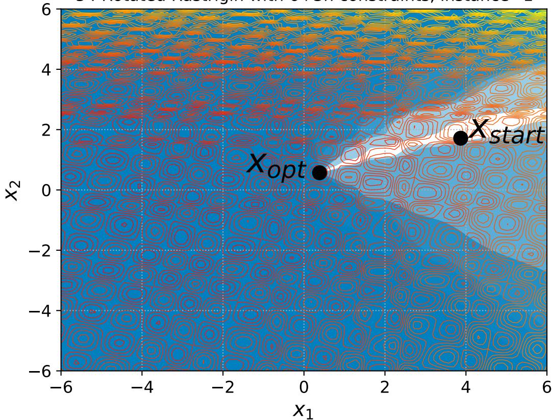
54 Rotated Rastrigin with 6+3n constraints, instance=1
