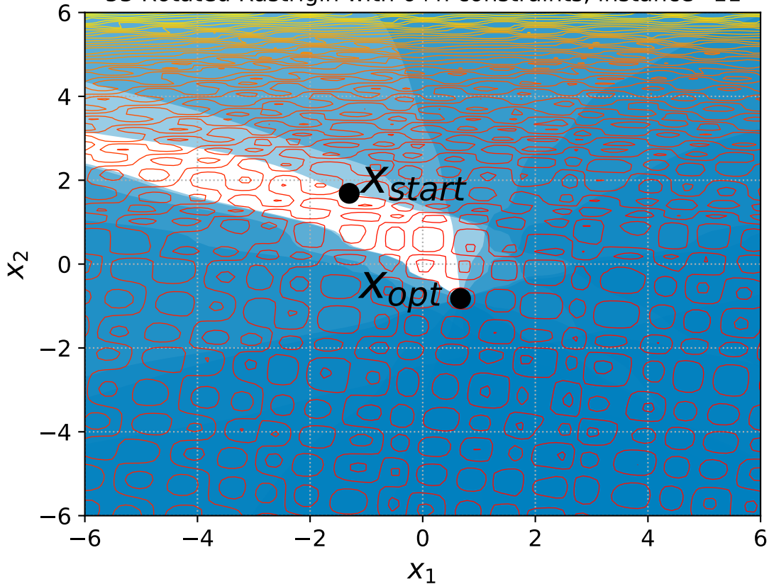
53 Rotated Rastrigin with 6+n constraints, instance=11
