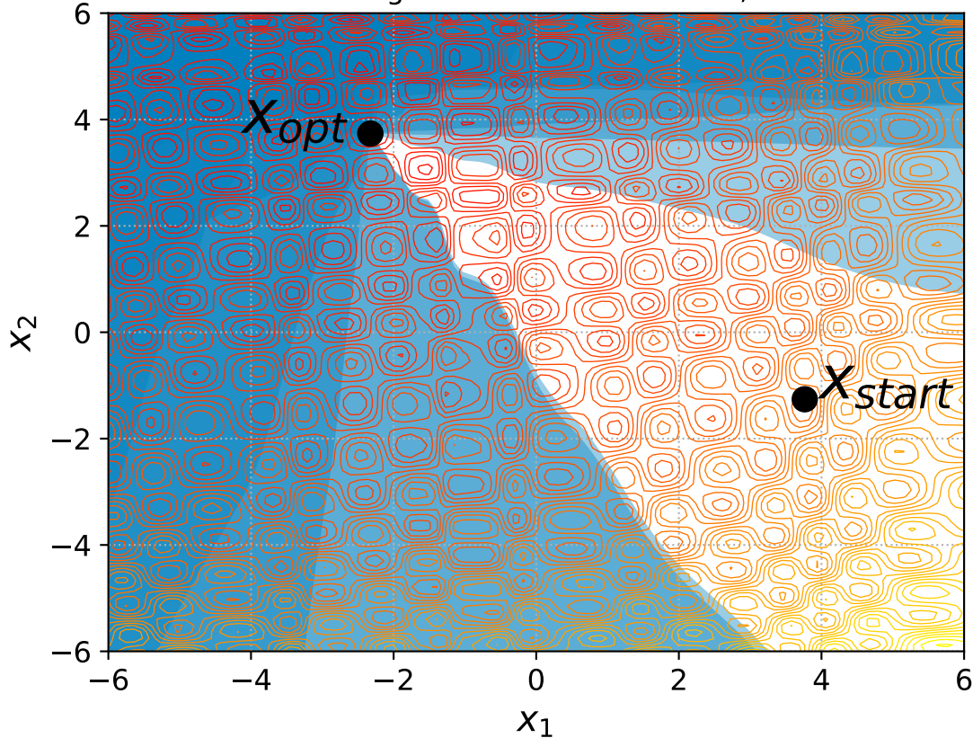
53 Rotated Rastrigin with 6+n constraints, instance=10
