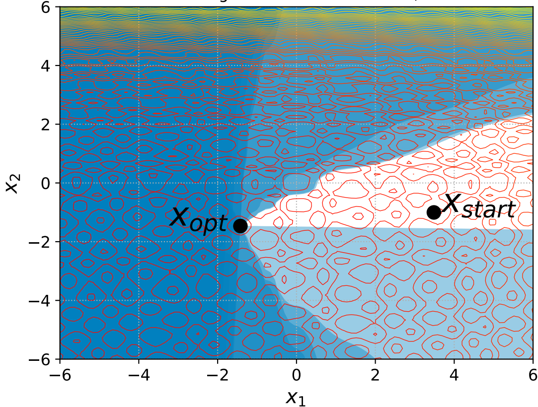
53 Rotated Rastrigin with 6+n constraints, instance=9
