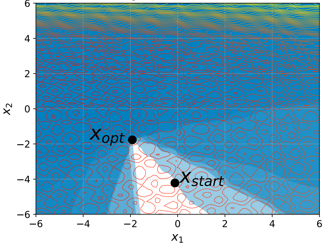
53 Rotated Rastrigin with 6+n constraints, instance=6
