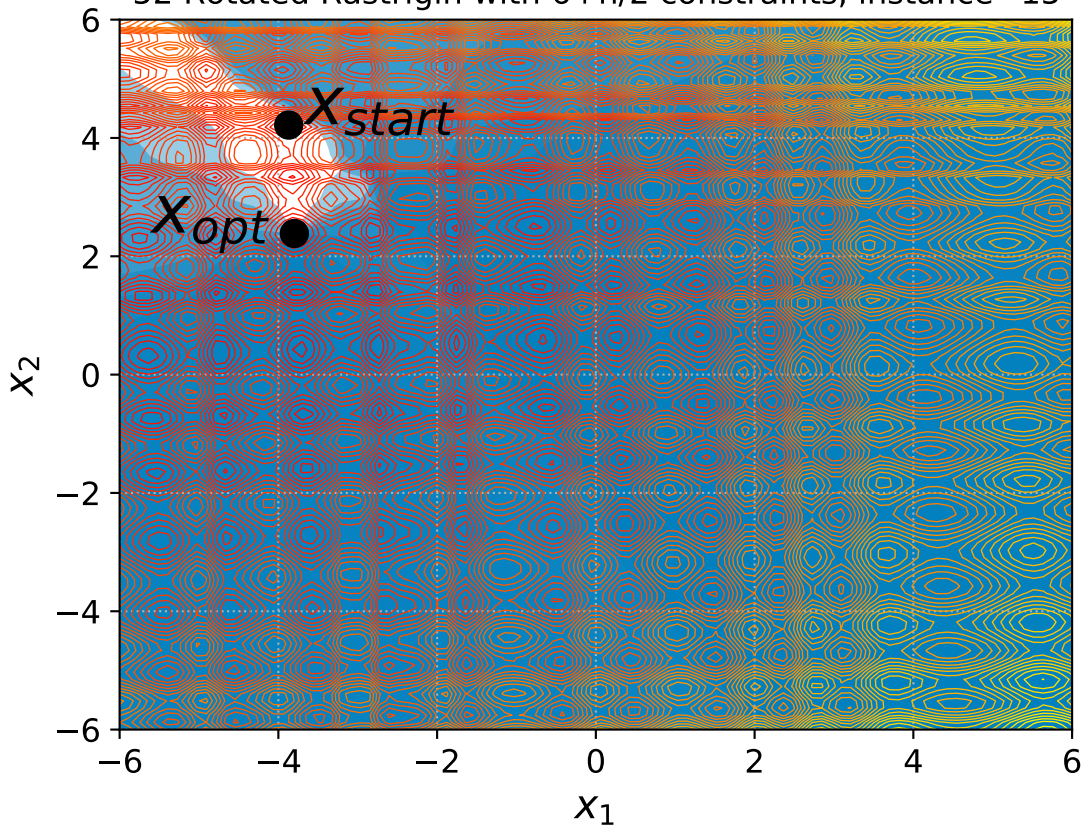
52 Rotated Rastrigin with 6+n/2 constraints, instance=15
