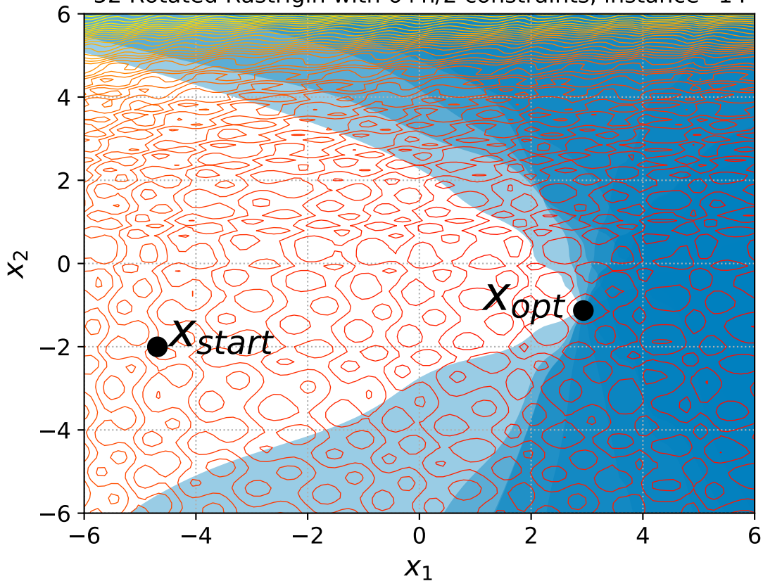
52 Rotated Rastrigin with 6+n/2 constraints, instance=14
