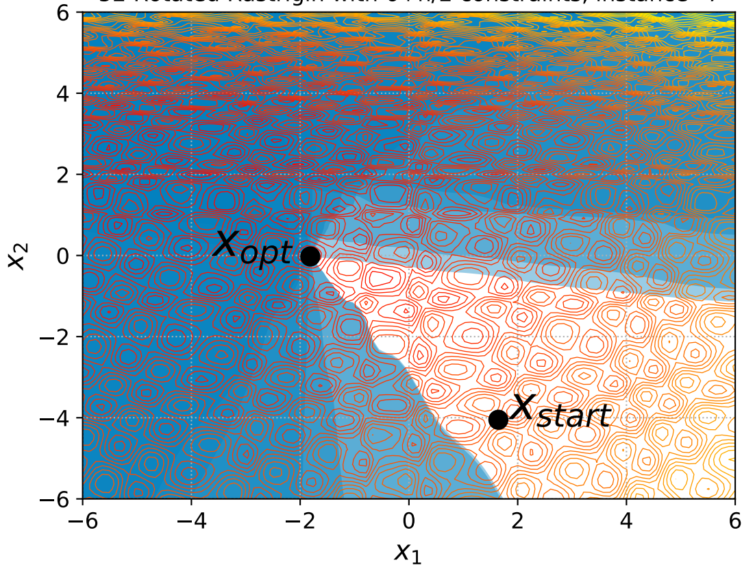
52 Rotated Rastrigin with 6+n/2 constraints, instance=7
