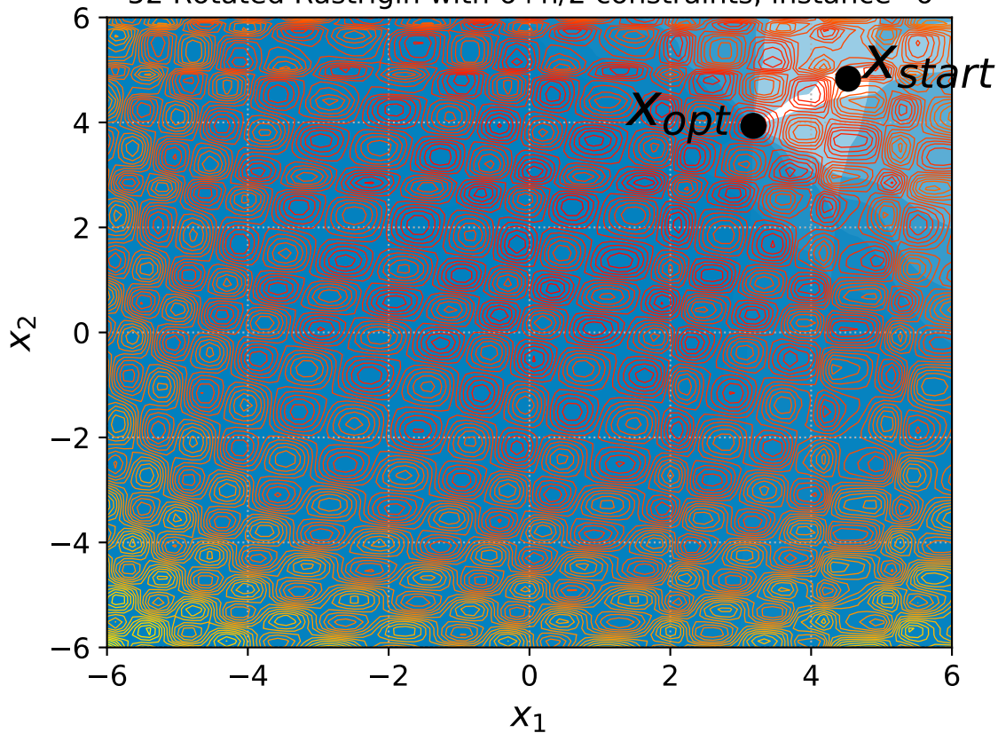
52 Rotated Rastrigin with 6+n/2 constraints, instance=6
