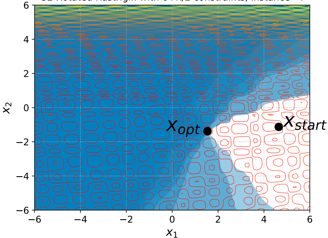
52 Rotated Rastrigin with 6+n/2 constraints, instance=4
