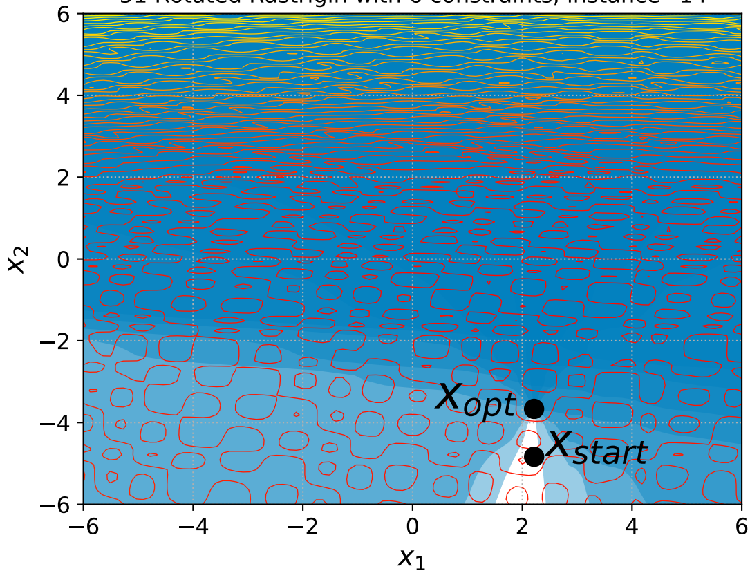
51 Rotated Rastrigin with 6 constraints, instance=14
