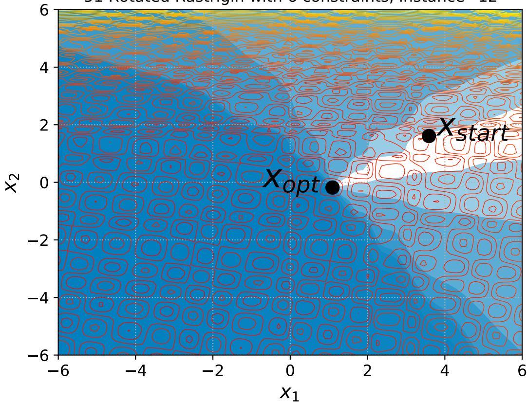
51 Rotated Rastrigin with 6 constraints, instance=12
