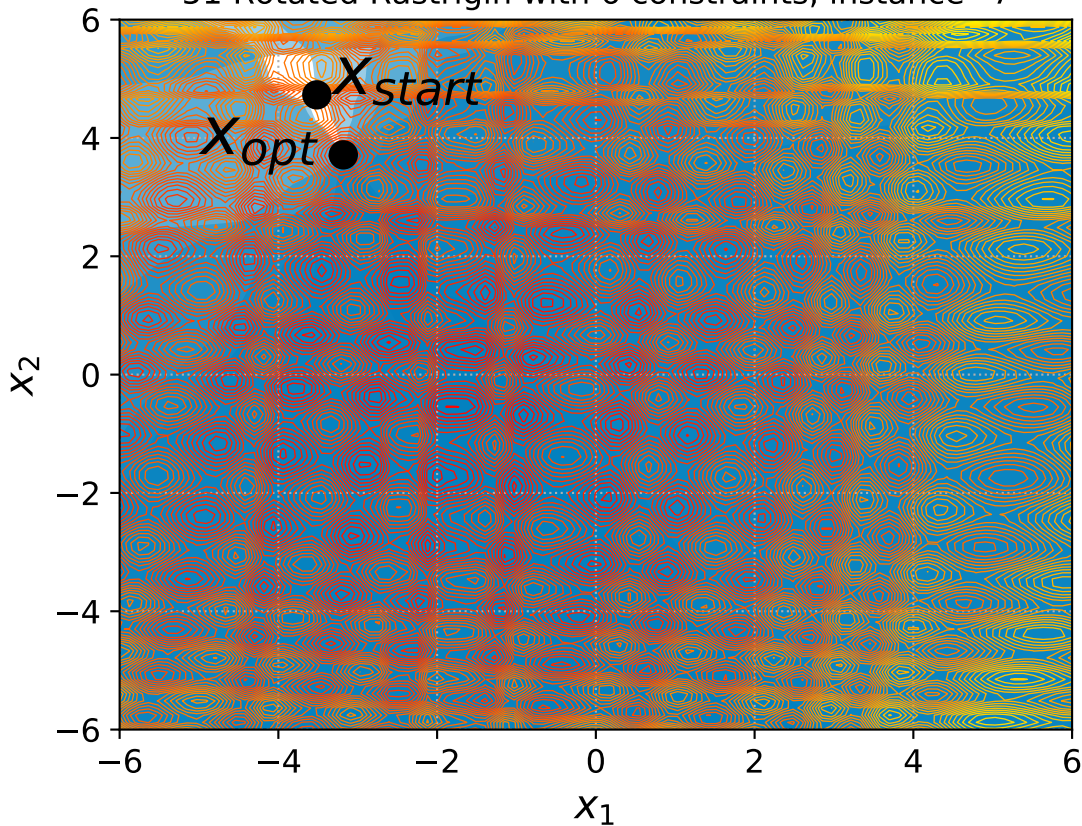
51 Rotated Rastrigin with 6 constraints, instance=7
