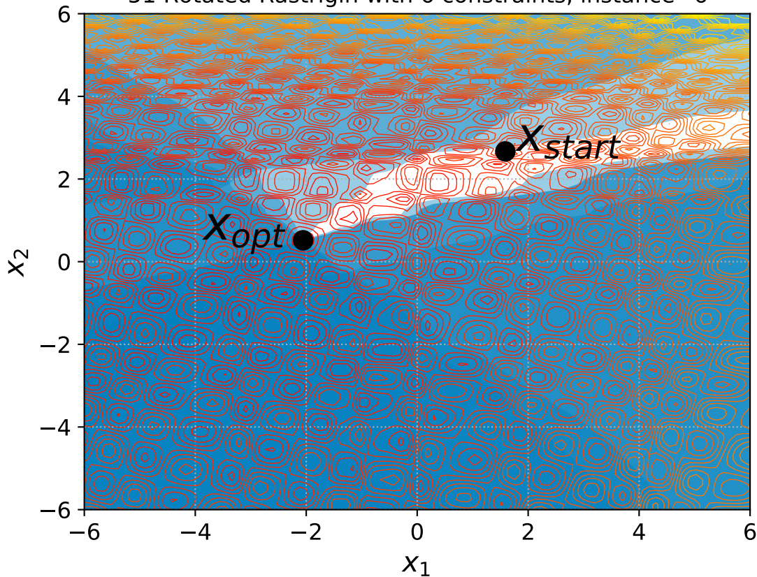
51 Rotated Rastrigin with 6 constraints, instance=6
