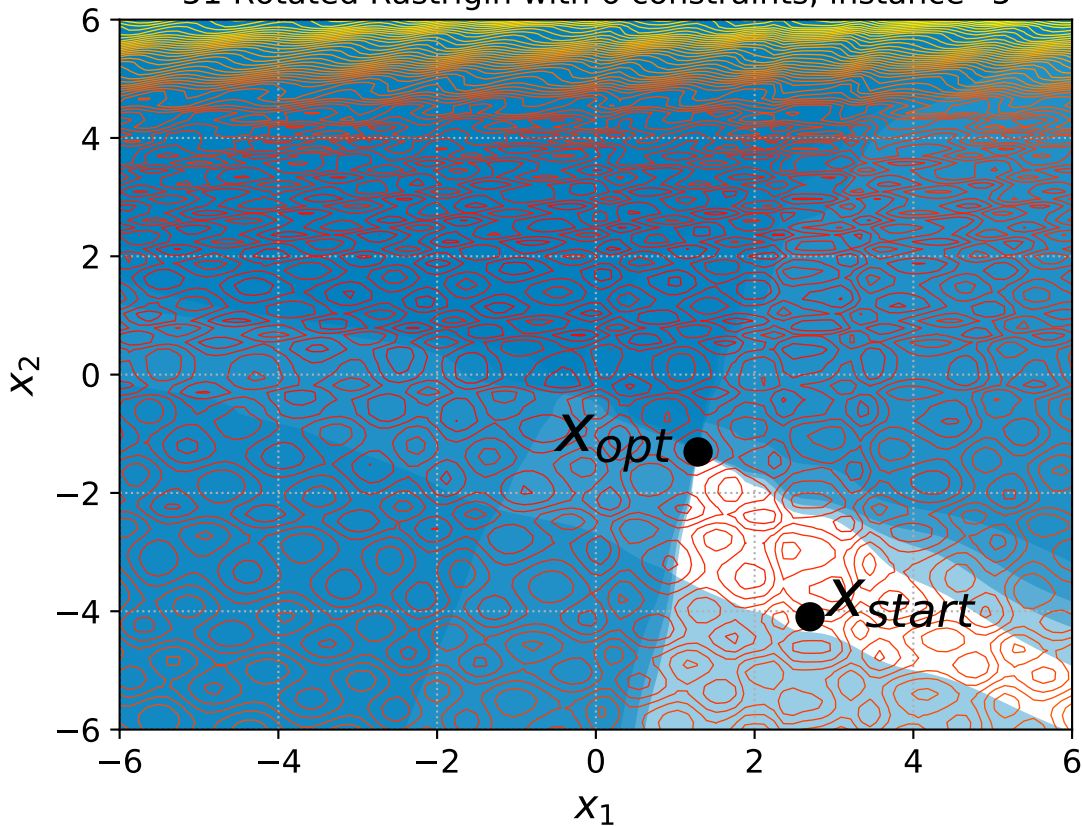
51 Rotated Rastrigin with 6 constraints, instance=5
