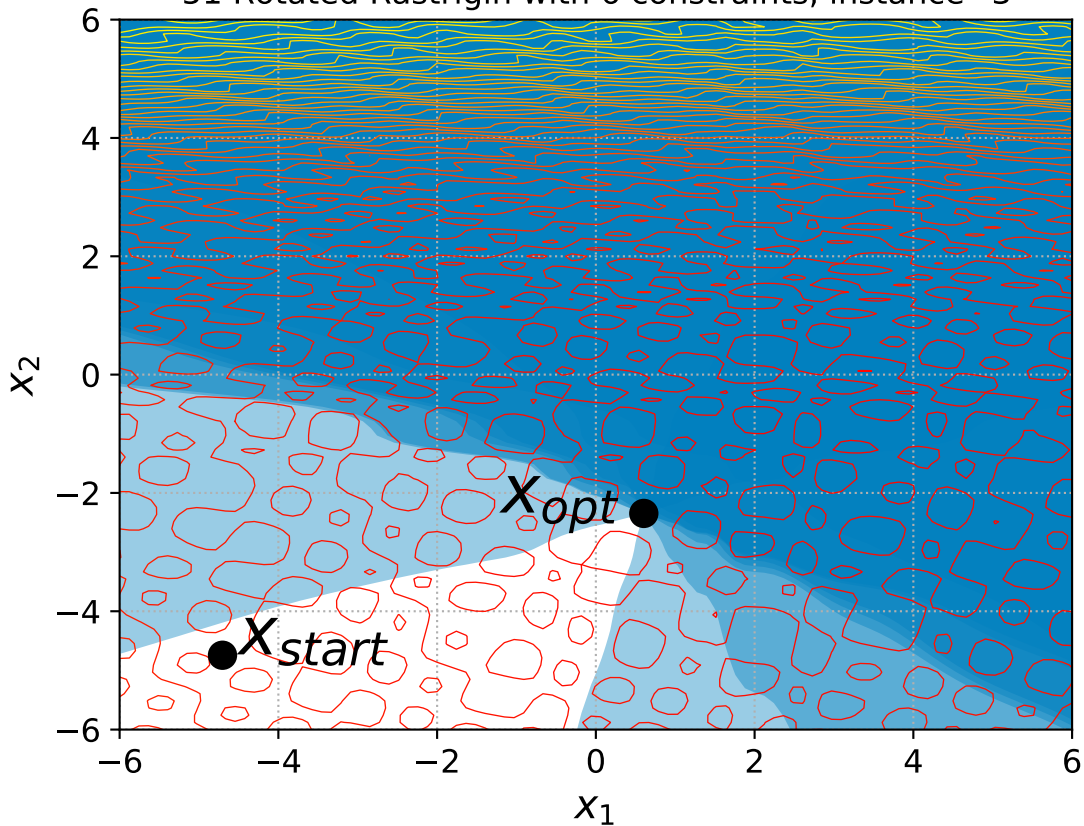
51 Rotated Rastrigin with 6 constraints, instance=3
