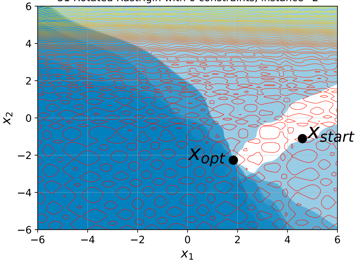
51 Rotated Rastrigin with 6 constraints, instance=2
