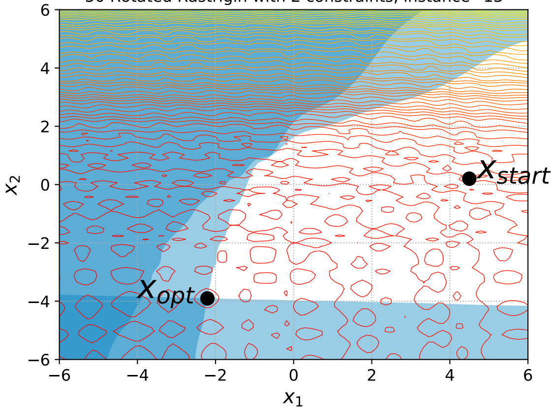
50 Rotated Rastrigin with 2 constraints, instance=13
