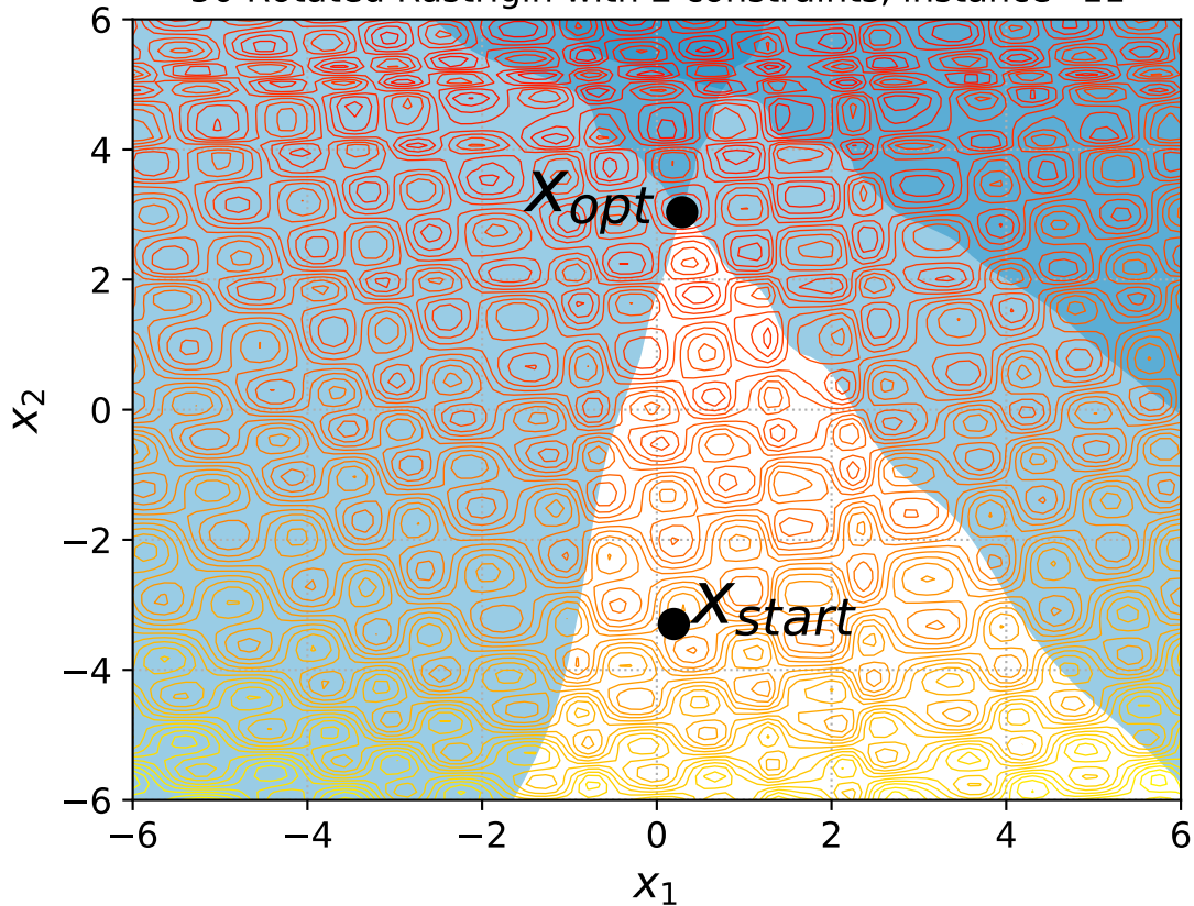
50 Rotated Rastrigin with 2 constraints, instance=11
