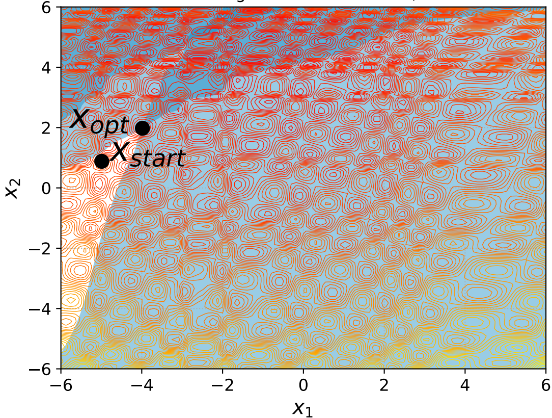
50 Rotated Rastrigin with 2 constraints, instance=9
