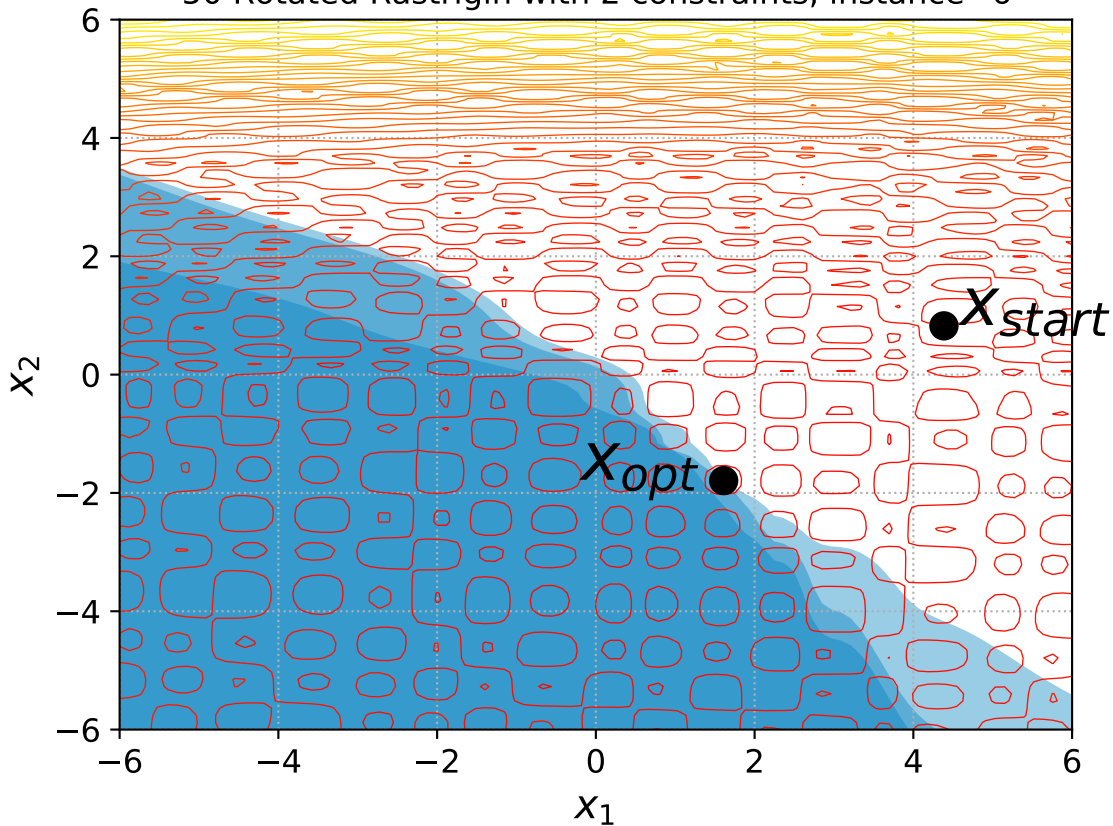
50 Rotated Rastrigin with 2 constraints, instance=6
