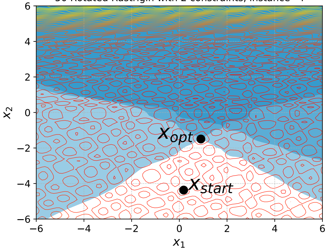
50 Rotated Rastrigin with 2 constraints, instance=4
