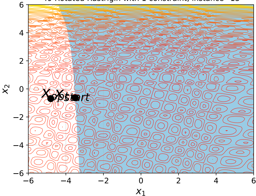
49 Rotated Rastrigin with 1 constraint, instance=13
