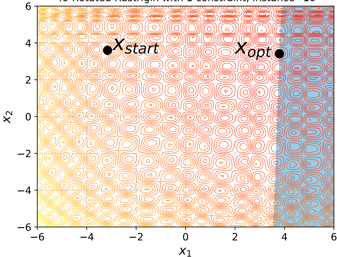
49 Rotated Rastrigin with 1 constraint, instance=10
