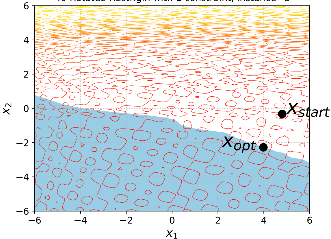
49 Rotated Rastrigin with 1 constraint, instance=8
