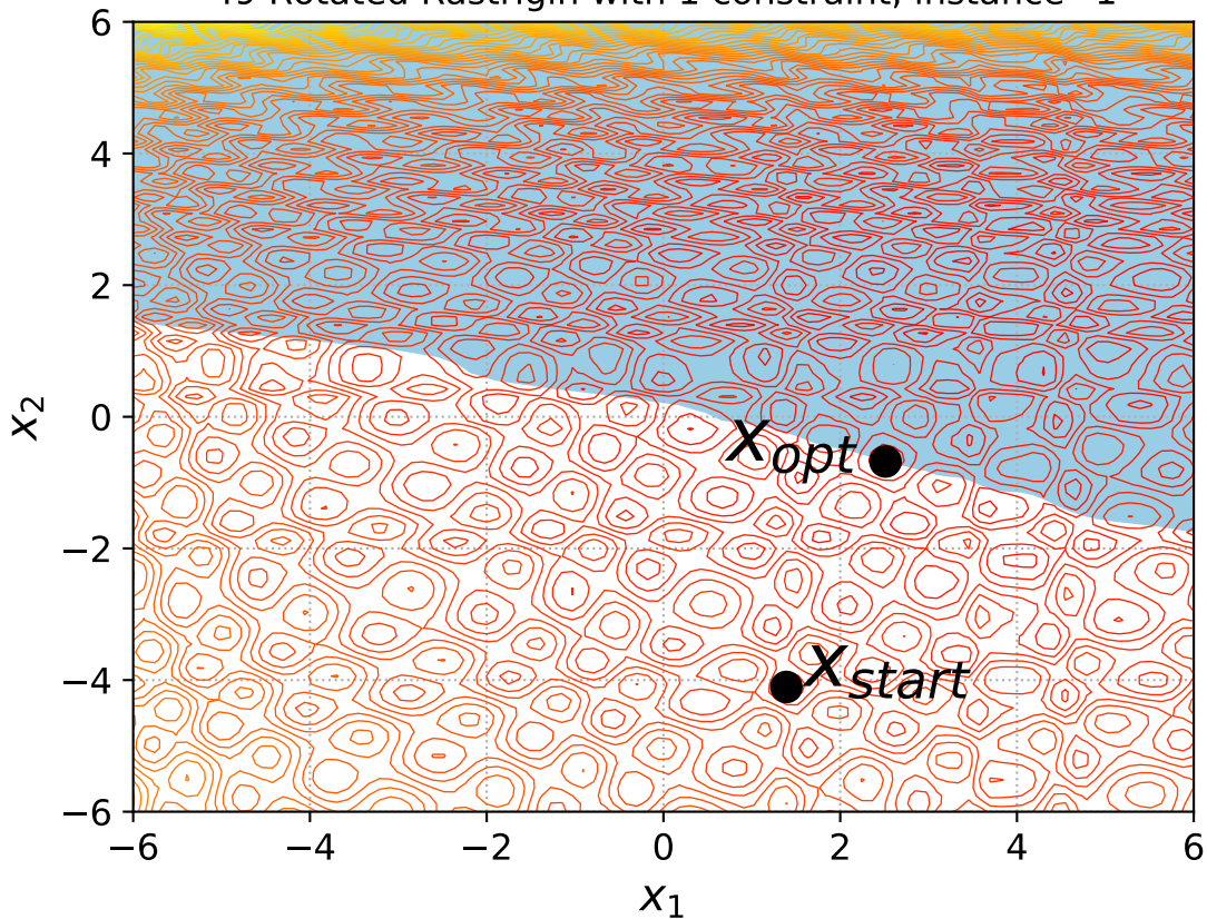
49 Rotated Rastrigin with 1 constraint, instance=1
