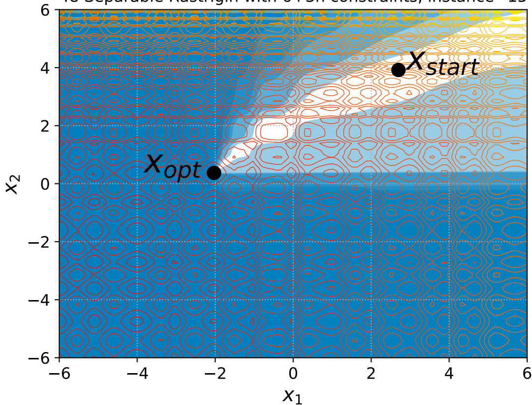
48 Separable Rastrigin with 6+3n constraints, instance=15
