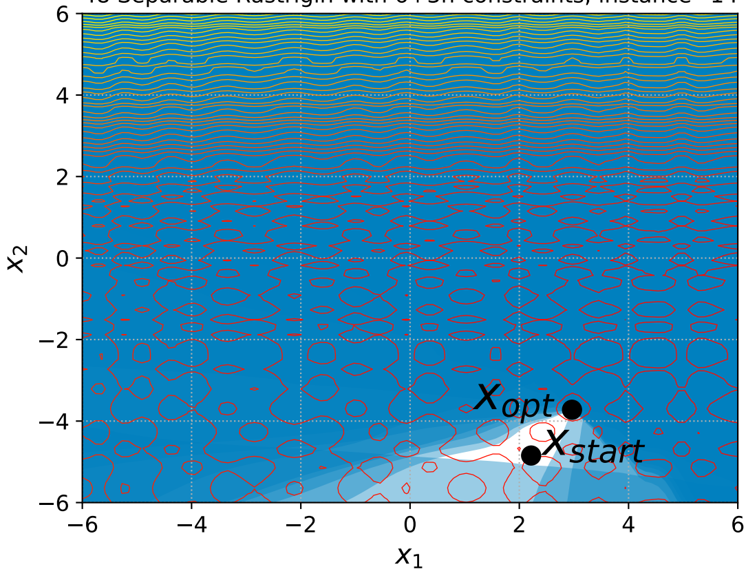
48 Separable Rastrigin with 6+3n constraints, instance=14
