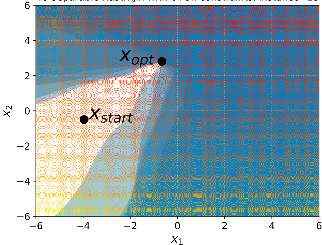
48 Separable Rastrigin with 6+3n constraints, instance=13
