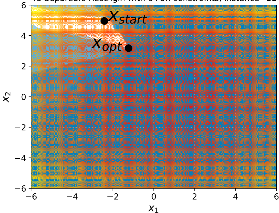
48 Separable Rastrigin with 6+3n constraints, instance=11
