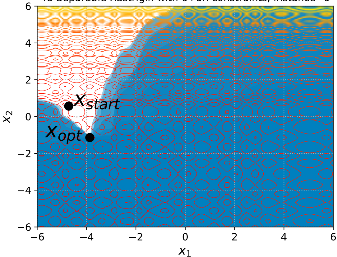
48 Separable Rastrigin with 6+3n constraints, instance=9
