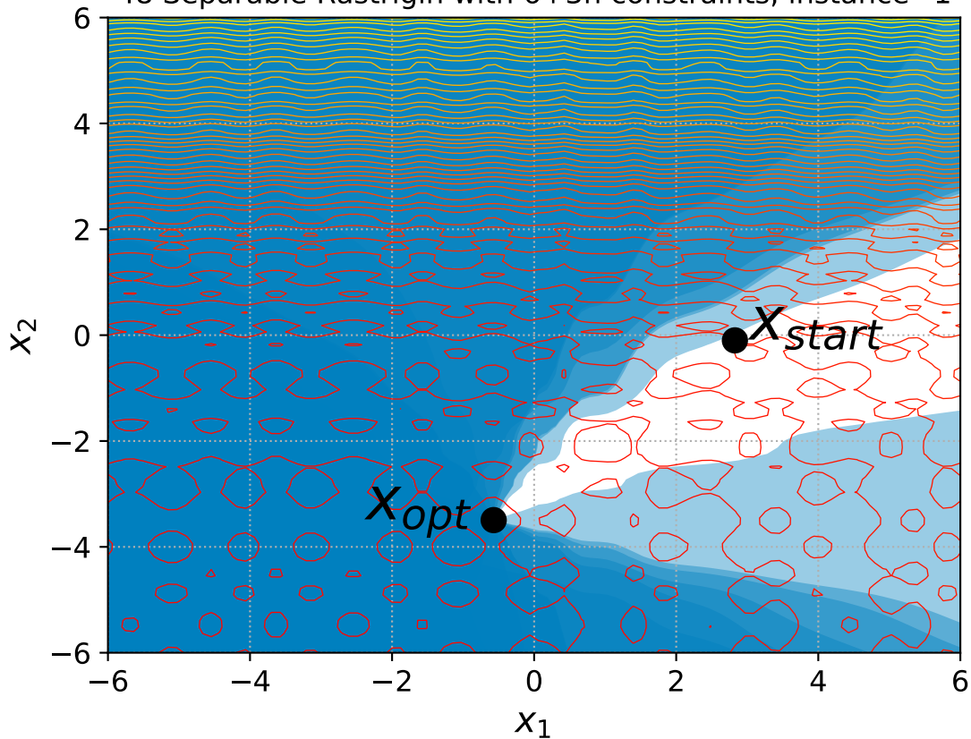
48 Separable Rastrigin with 6+3n constraints, instance=1
