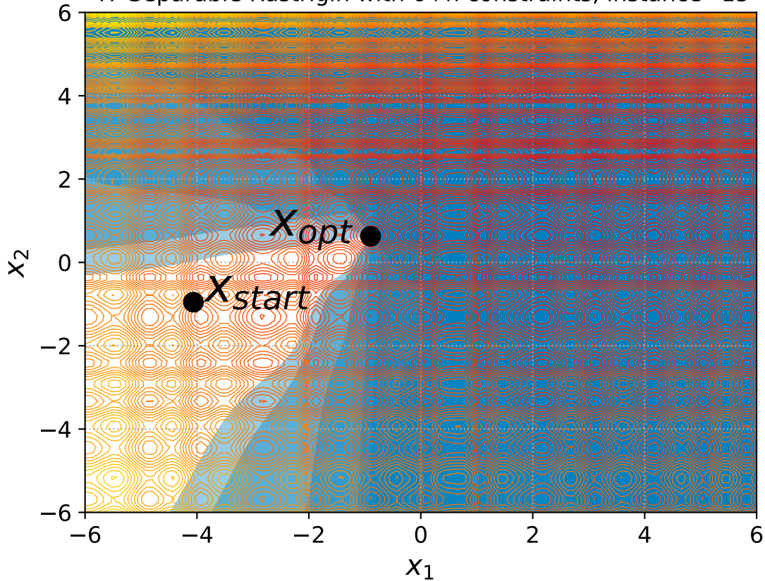
47 Separable Rastrigin with 6+n constraints, instance=15
