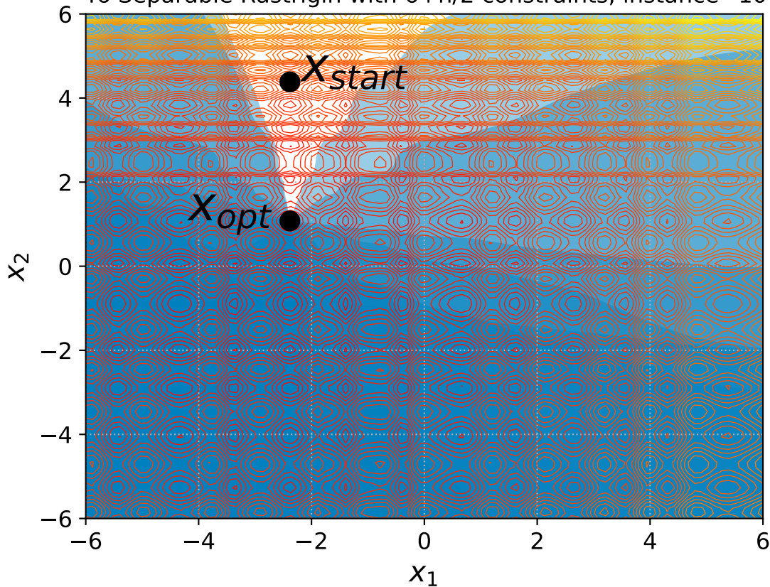
46 Separable Rastrigin with 6+n/2 constraints, instance=10
