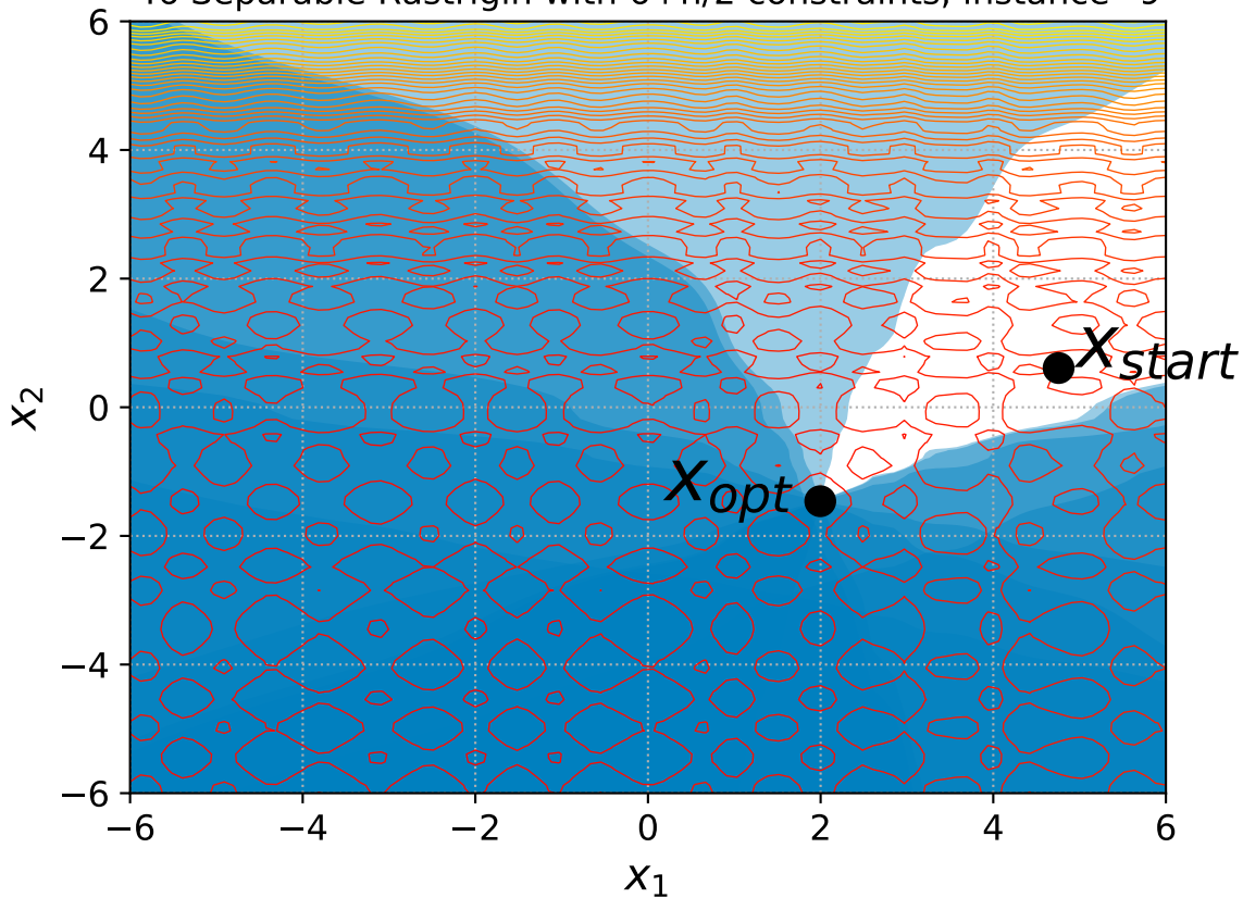
46 Separable Rastrigin with 6+n/2 constraints, instance=9
