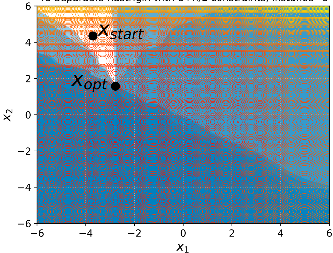
46 Separable Rastrigin with 6+n/2 constraints, instance=6
