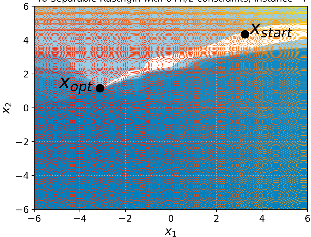
46 Separable Rastrigin with 6+n/2 constraints, instance=4
