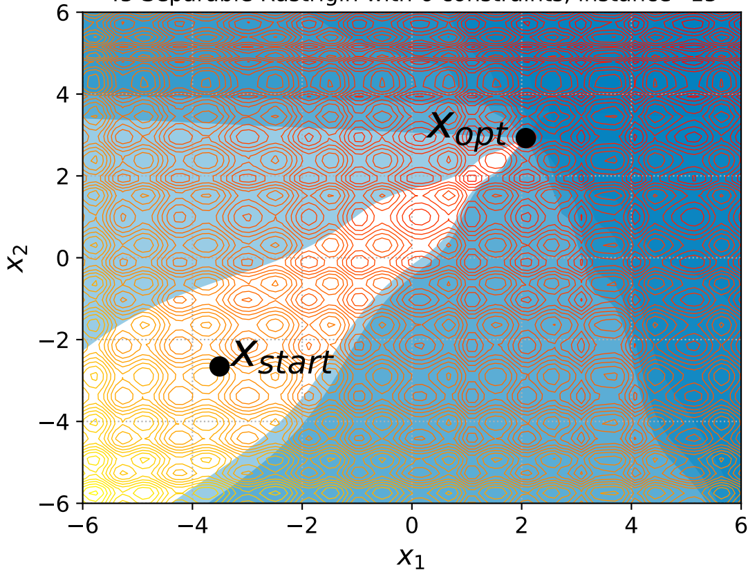
45 Separable Rastrigin with 6 constraints, instance=15
