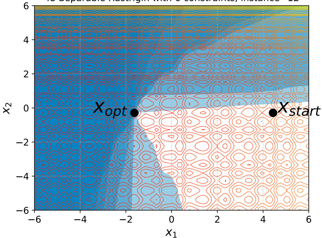
45 Separable Rastrigin with 6 constraints, instance=12
