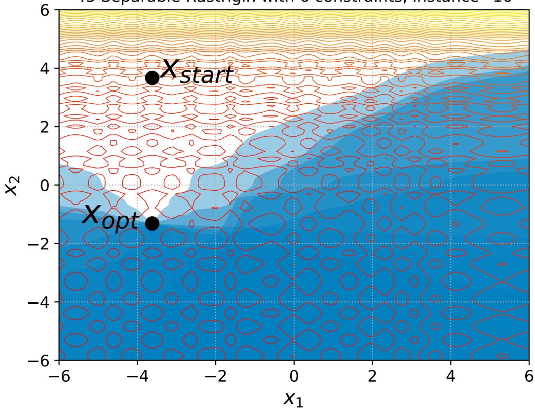
45 Separable Rastrigin with 6 constraints, instance=10
