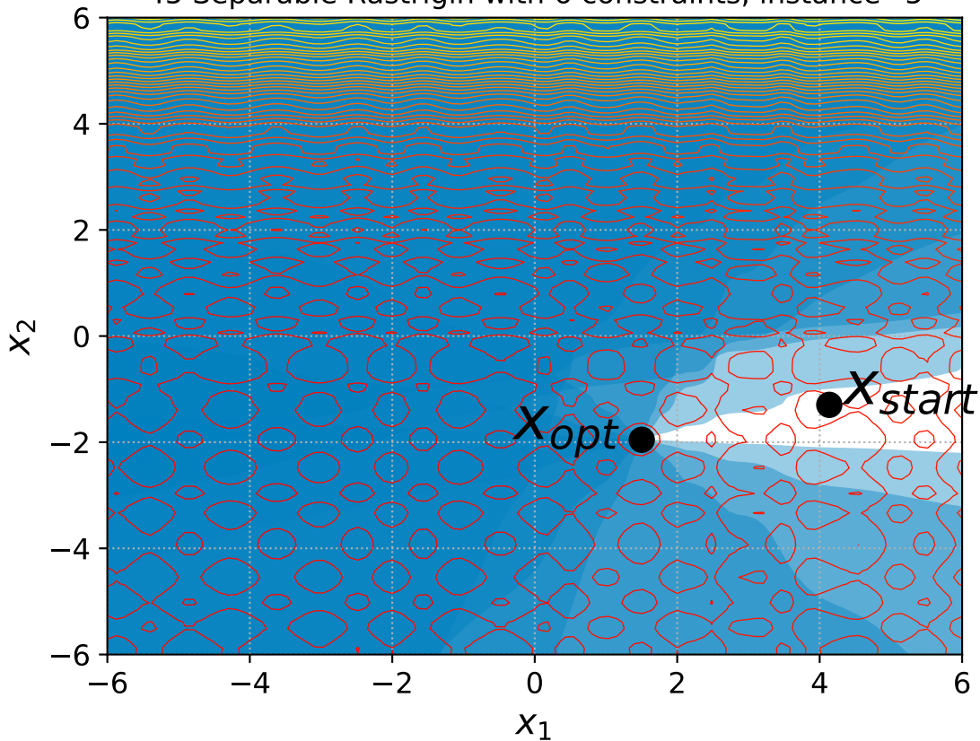
45 Separable Rastrigin with 6 constraints, instance=5
