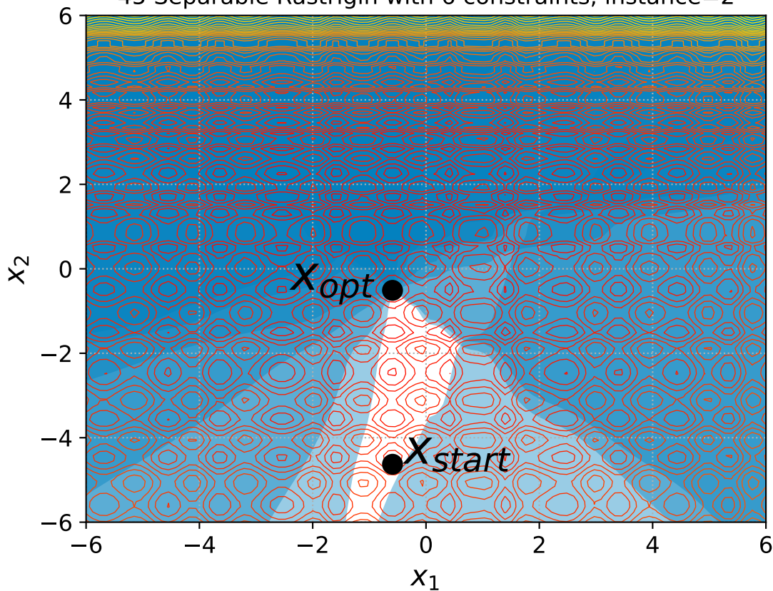
45 Separable Rastrigin with 6 constraints, instance=2
