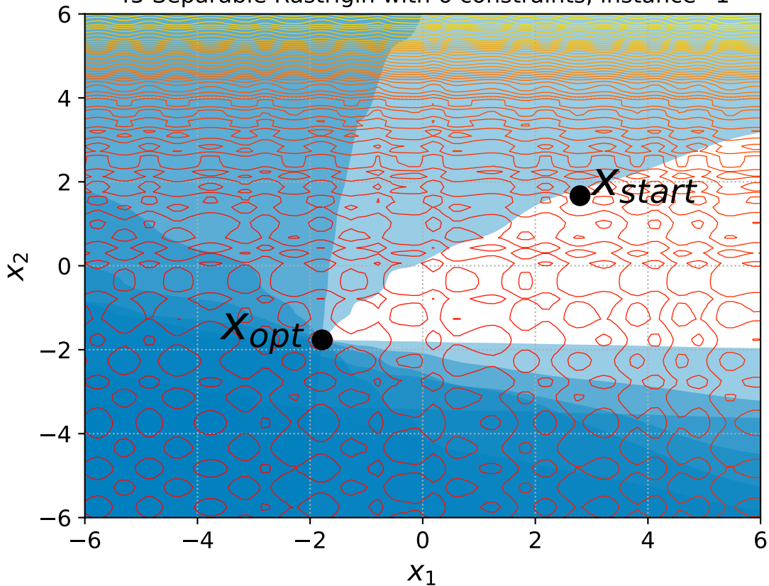
45 Separable Rastrigin with 6 constraints, instance=1
