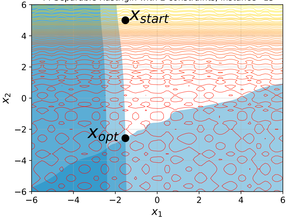
44 Separable Rastrigin with 2 constraints, instance=15
