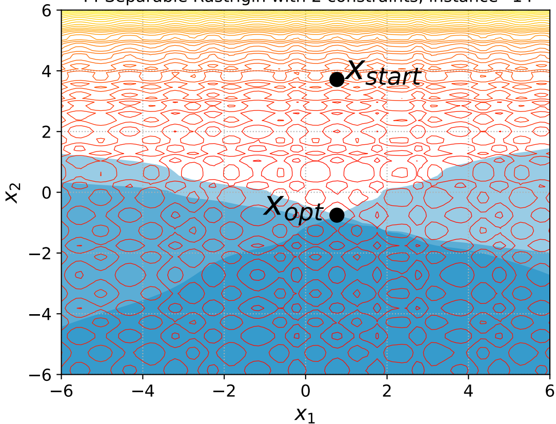
44 Separable Rastrigin with 2 constraints, instance=14
