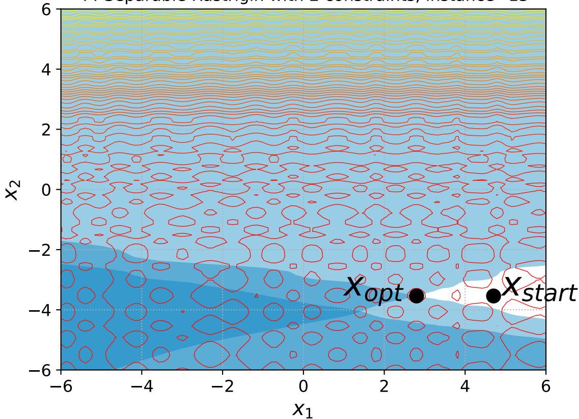
44 Separable Rastrigin with 2 constraints, instance=13
