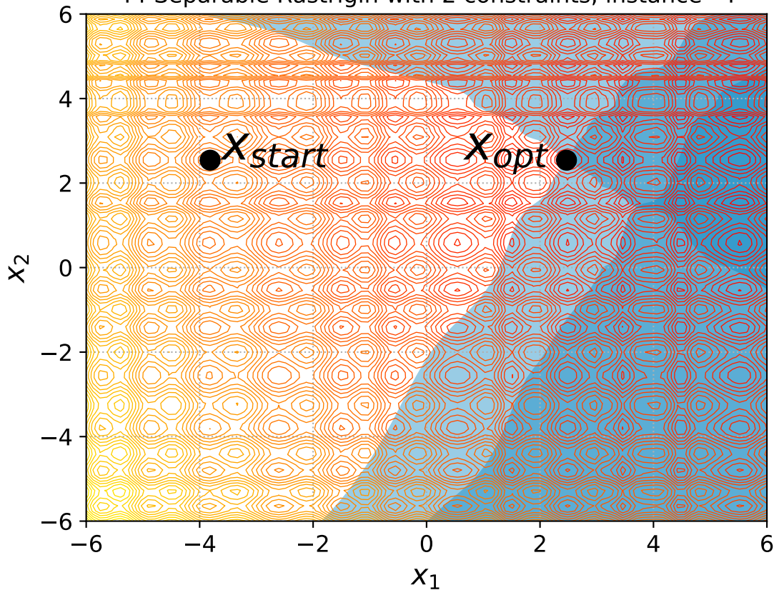
44 Separable Rastrigin with 2 constraints, instance=4
